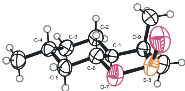
Figure 1. Graphical representation of X-ray crystal structure of sultine 6 .
